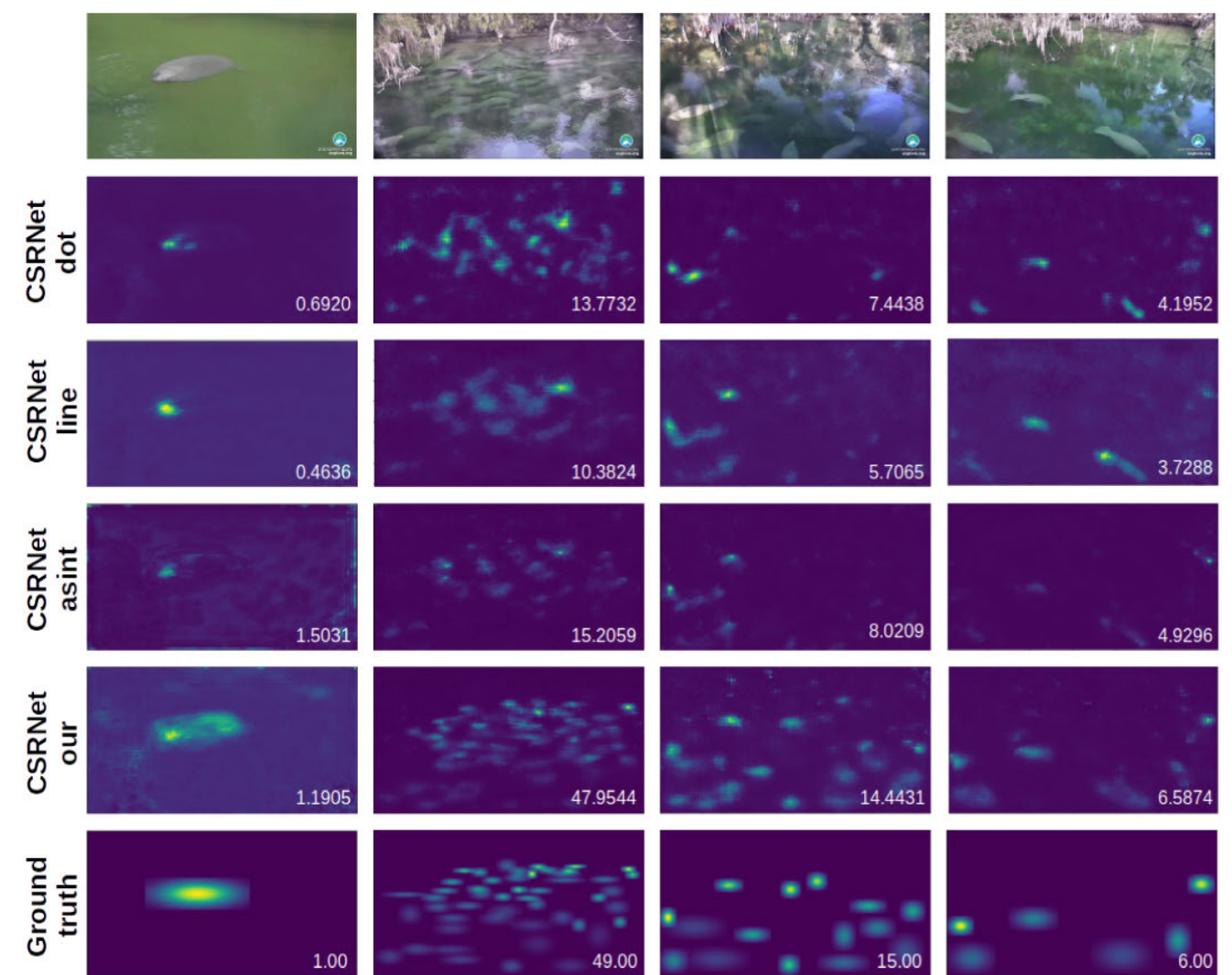
FIGURE 8. Comparison of density maps from the test set using the state-of-the-art CSRNet models (dot, lines, and Anisotropic Gaussian), our and the ground truth generated with the 2-D Gaussian kernel function.
