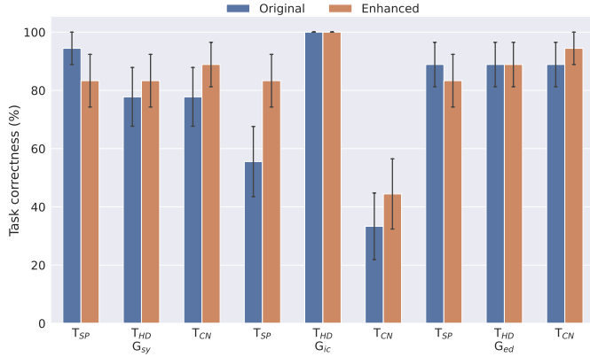
Fig. 2. Average task correctness across task types and graphs. Error bars indicate the standard error. Original: the single-layer graphs in Study 1, Enhanced: the gaze-enhanced graphs in Study 3 (Section VI).
