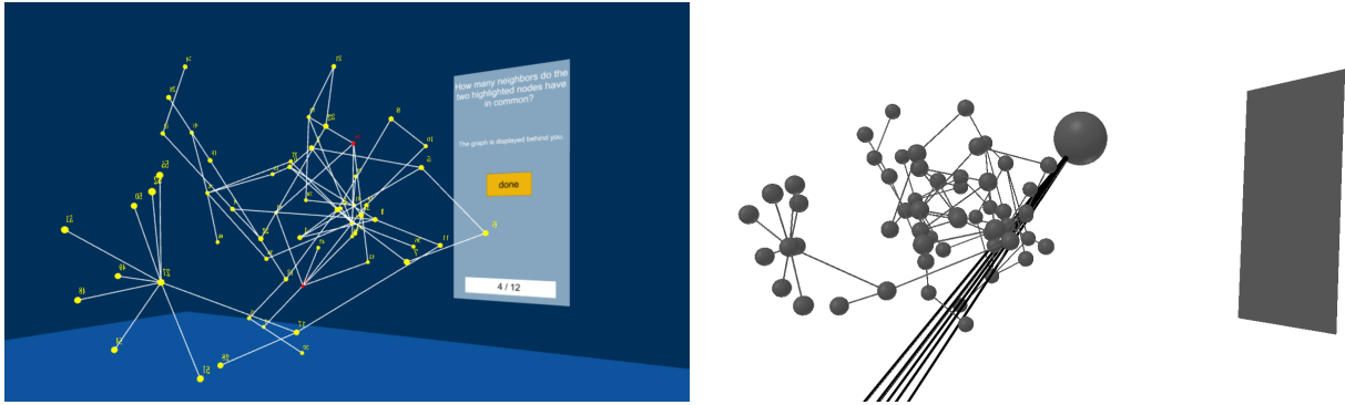
Fig. 1. Left: Our immersive environment displaying a 3D graph with highlighted nodes shown in red for the common neighbours task ( T_{CN} ). The question panel displays the task instruction and progress indicator. Right: Visualisation of the perspective reconstruction and ray casting. The large sphere represents the camera position. A cone of nine rays emanates from the camera origin. The black rectangular plane represents the question panel.
