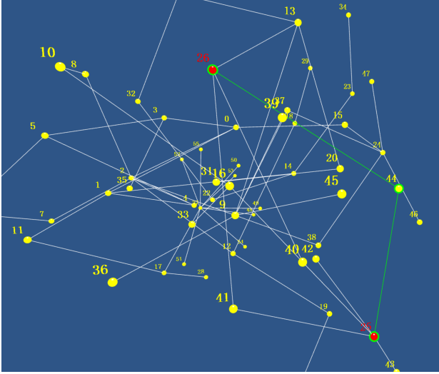
Fig. 6. The gaze-enhanced visual representation under G_{ic} , T_{CN} . Cued task-relevant nodes and edges, derived from the gaze patterns of successful ( pos -group) analysts, are emphasised with green outlines.
