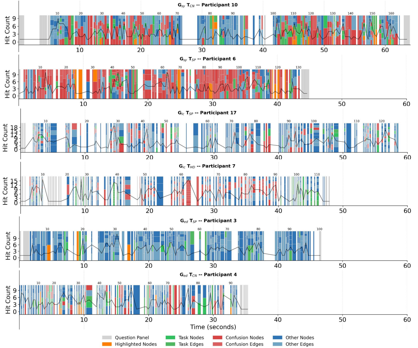
Fig. 4. Sample timeline (scarf-plot) visualisations of gaze behaviour, enlarged to full width for legibility. Each vertical bar represents a fixation event, with width indicating duration and coloured blocks representing the AOIs that intersected the eye-gaze ray; colours follow the eight-category AOI scheme of Section III-E. Within each block, objects are stacked from closest (bottom) to farthest (top).
