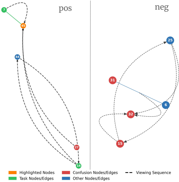
Fig. 5. Precedence state diagrams for the \text{Graph}_{ed} under task shortest path, showing the top 5 differentially frequent patterns for the pos -group (left) and neg -group (right).
