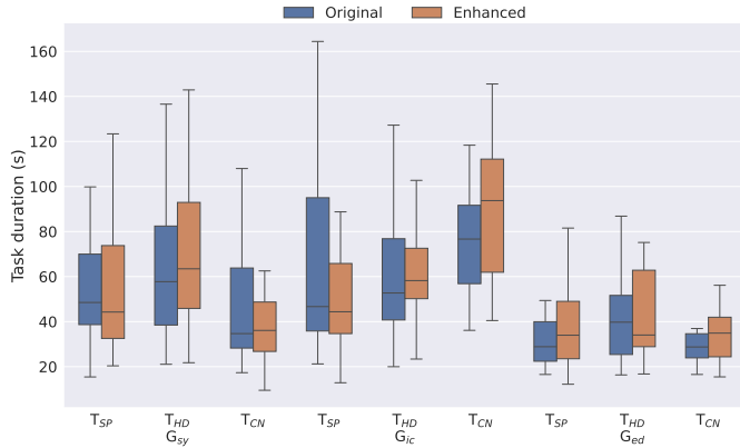
Fig. 3. Task duration for the original (Study 1) and enhanced (Study 3) conditions across various task types and graph datasets. The boxes span the first to third quartiles, with the median indicated by the centre line.
