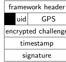
Figure 3. The identification header composed of the framework and application header.
